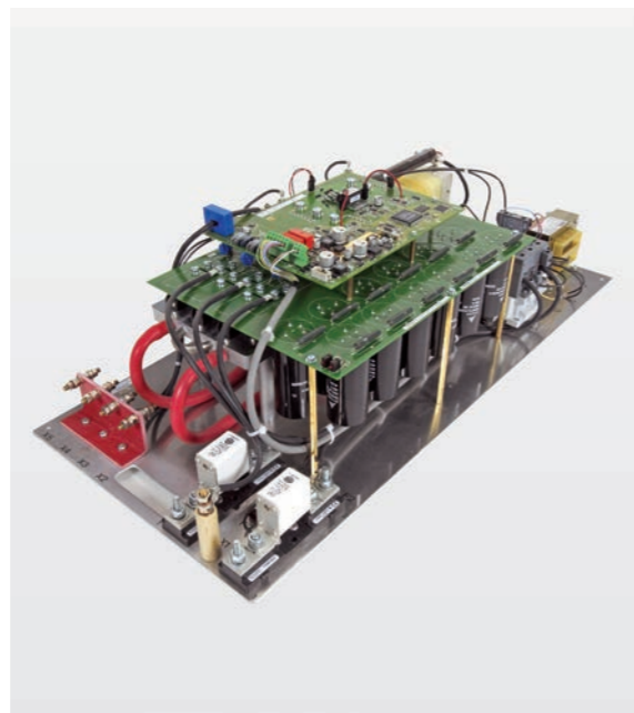
Water-cooled PSM9 Module.
